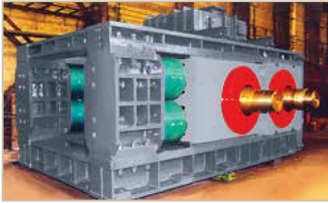
Roller Press Roll System
